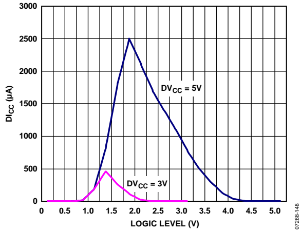
Figure 48. D_{CC} vs. Logic Input Voltage
